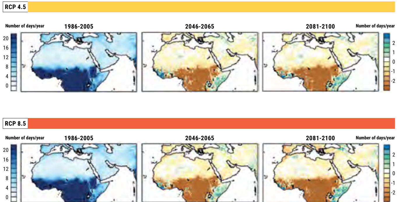
FIGURE 30: Mean change in the maximum length of wet spell (CWD) (days/yr) for mid- and end-century for ensemble of three RCP 4.5 and RCP 8.5 projections compared to the reference period
