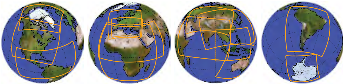
FIGURE 15: CORDEX domains
