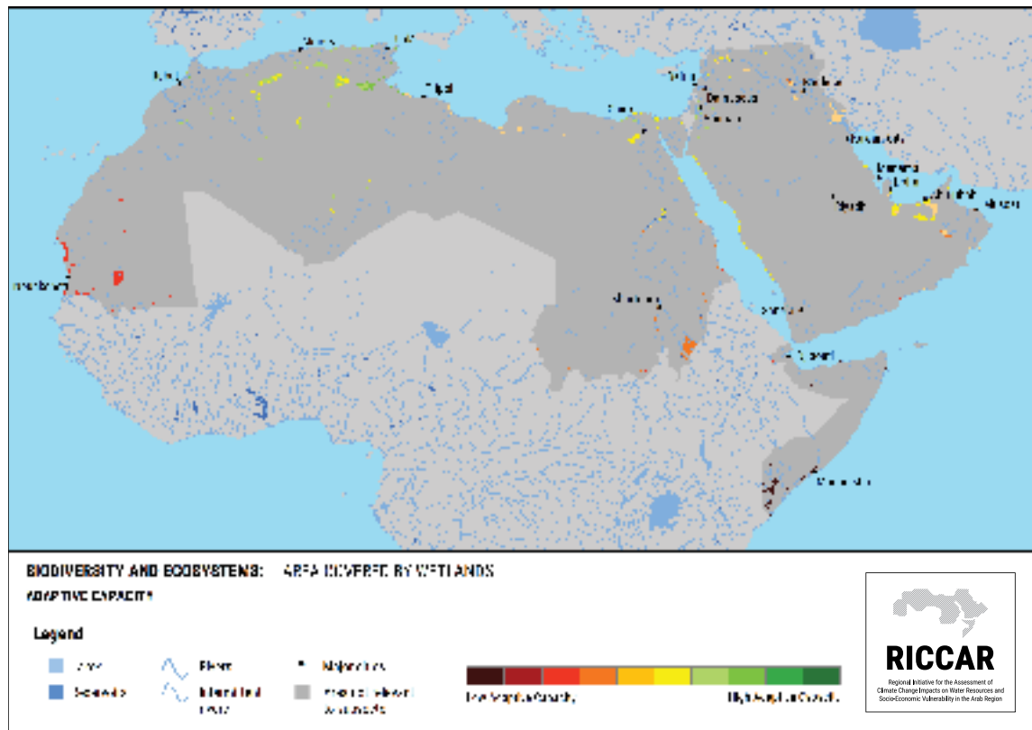
FIGURE 134: Area covered by wetlands – Adaptive capacity
