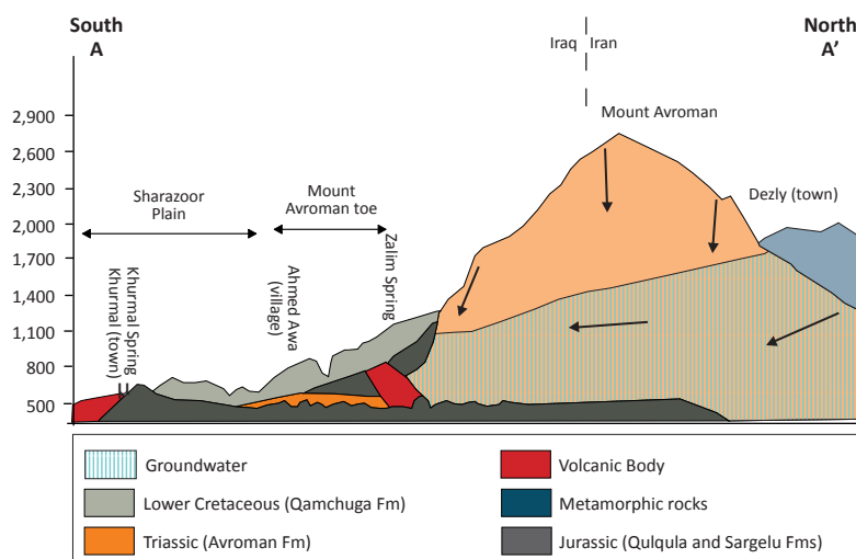
Figure 2. Geological cross-section of Mount Avroman and the Zalim Spring
