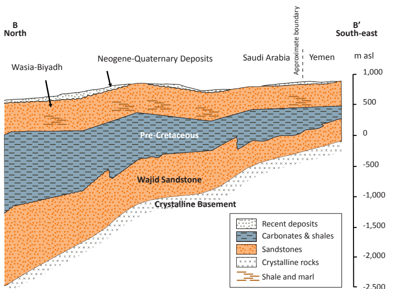
Figure 2. Geological cross-section of the Wajid Sandstones across the border of Saudi Arabia and Yemen
