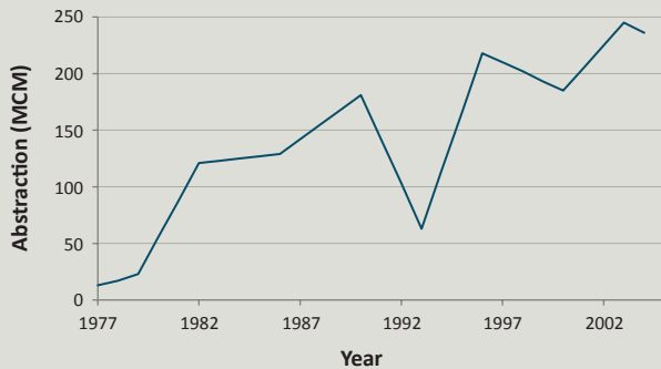
Figure 6. Historical abstraction in Najran in Saudi Arabia (1977-2004)
