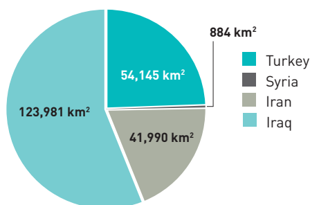
Figure 2. Distribution of the Tigris Basin area
