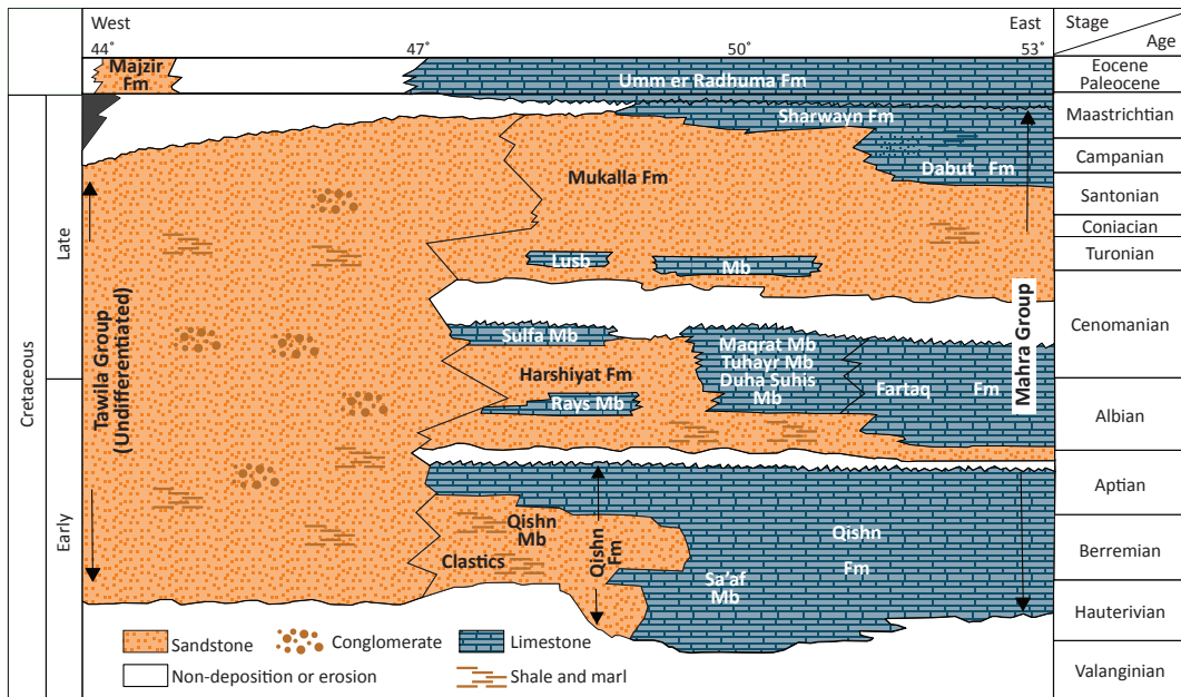
Figure 2. Lithostratigraphy of the Wasia-Biyadh-Aruma Aquifer System (South) in Yemen
