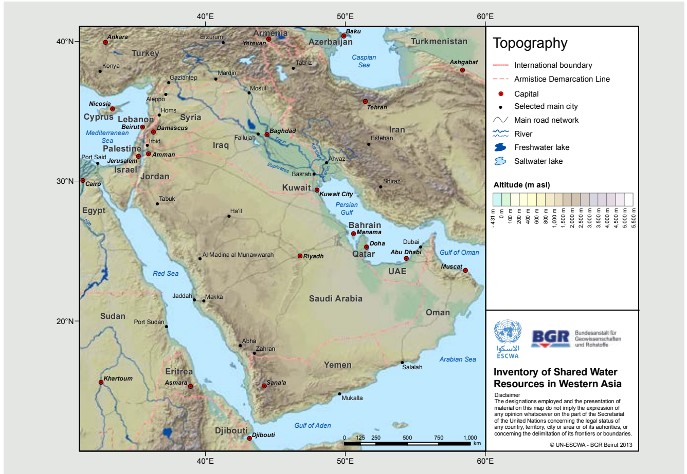
Figure 2. Topography of the Western Asia Region
