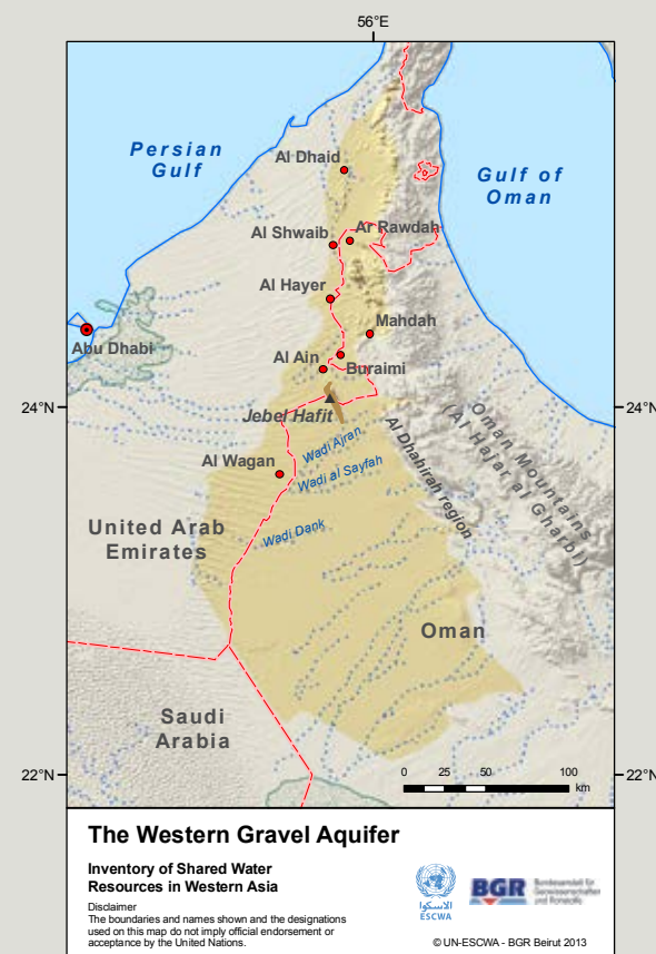
Figure 3. The Western Gravel Aquifer
