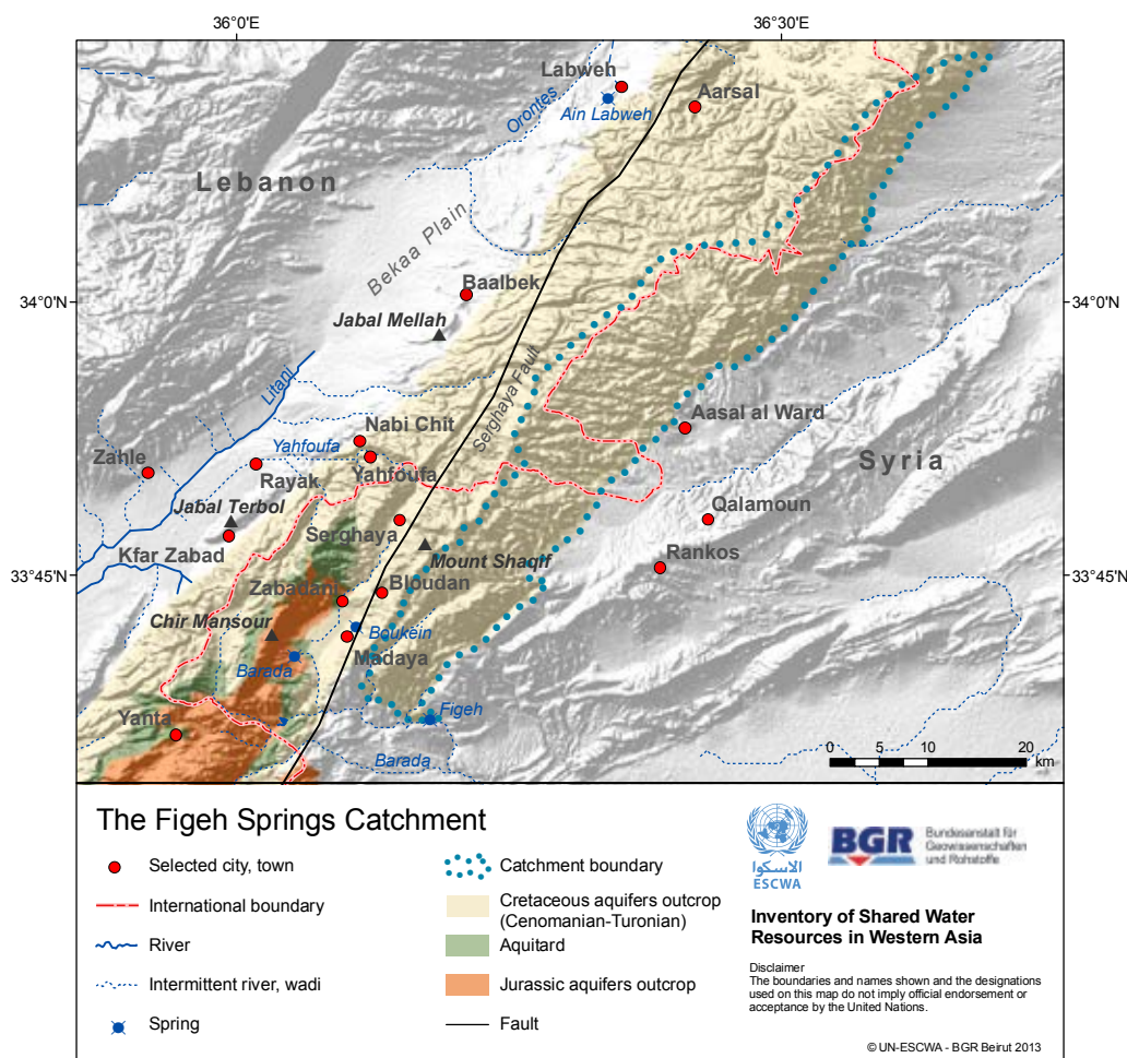
Figure 3. Overview Map of the FigeH Springs protection zone
