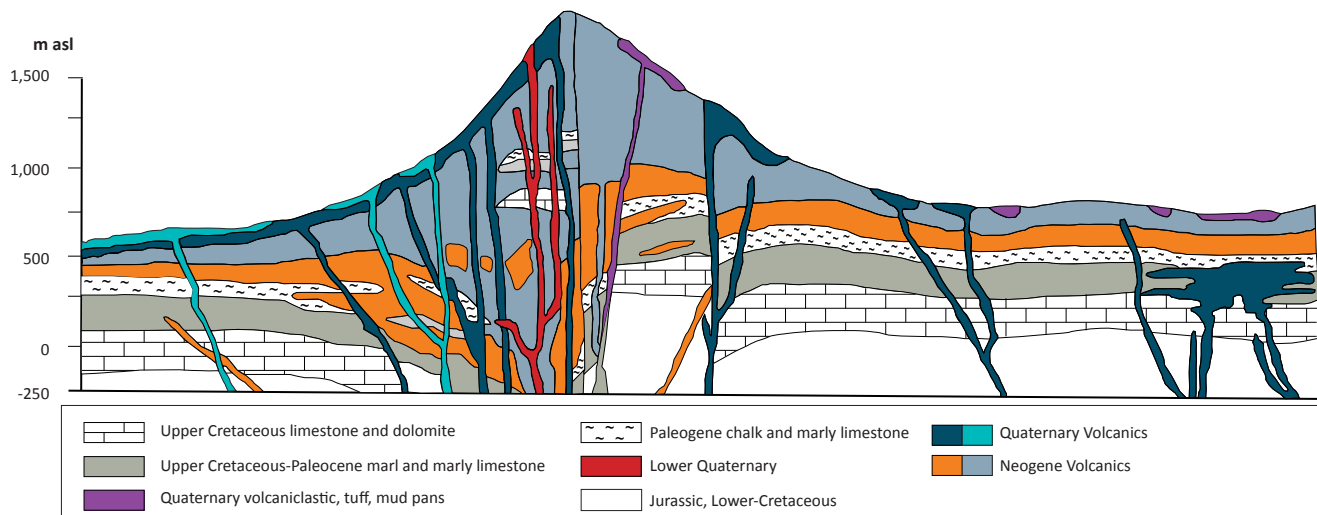
Figure 1. Schematic geological cross-section through the Jebel al Arab Mountain range
