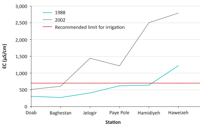
Figure 6. Changes in mean Electrical Conductivity (EC) values along the Karkheh River (1988 and 2002)
