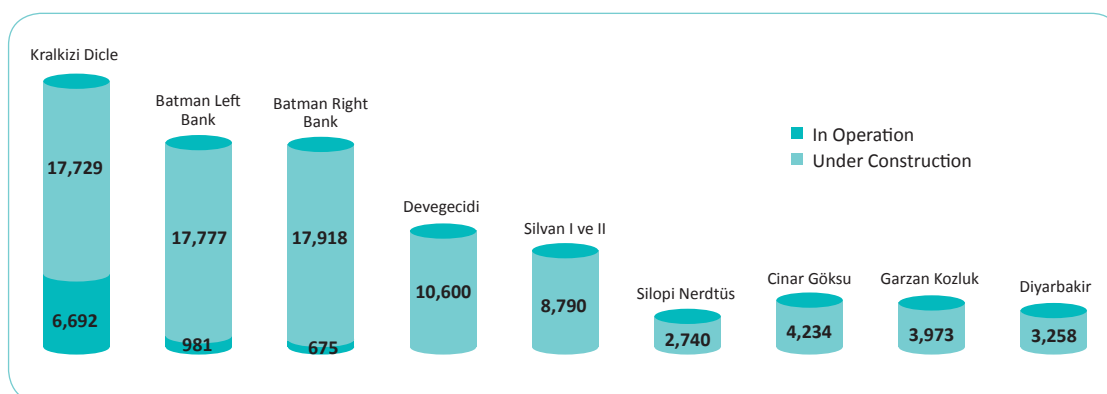
Figure 8. Irrigated area as part of GAP in the Tigris Basin in Turkey (ha)
