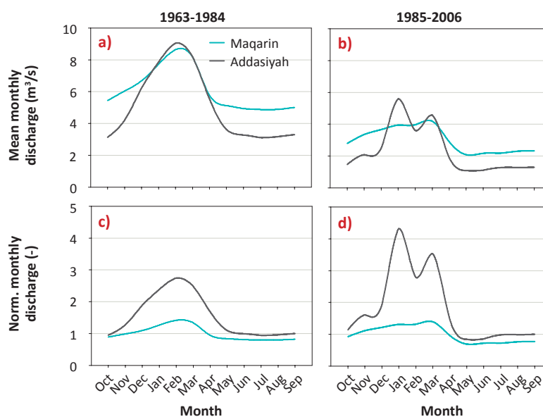
Figure 15. Mean monthly flow regime of the Yarmouk River at different gauging stations in Jordan (1963-2006)
