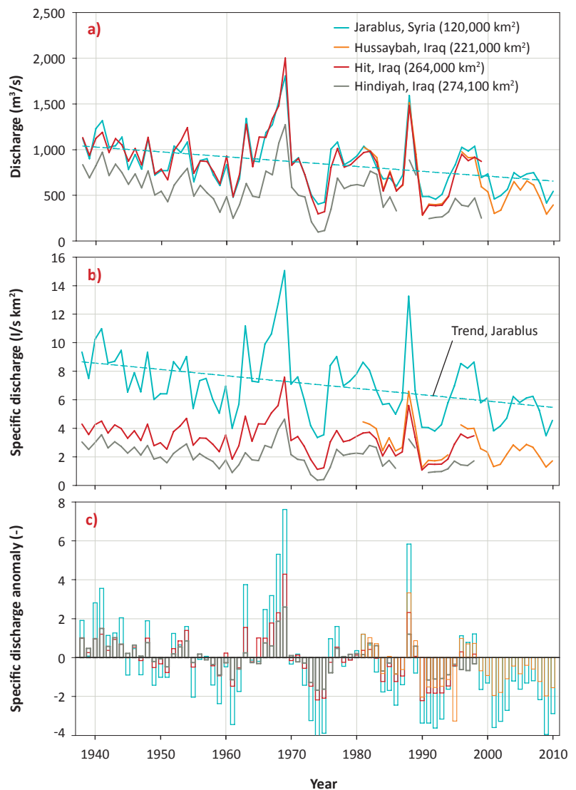
Figure 5. a) Mean annual discharge, b) specific mean annual discharge and c) discharge anomaly time series of the Euphrates (1937-2010)
