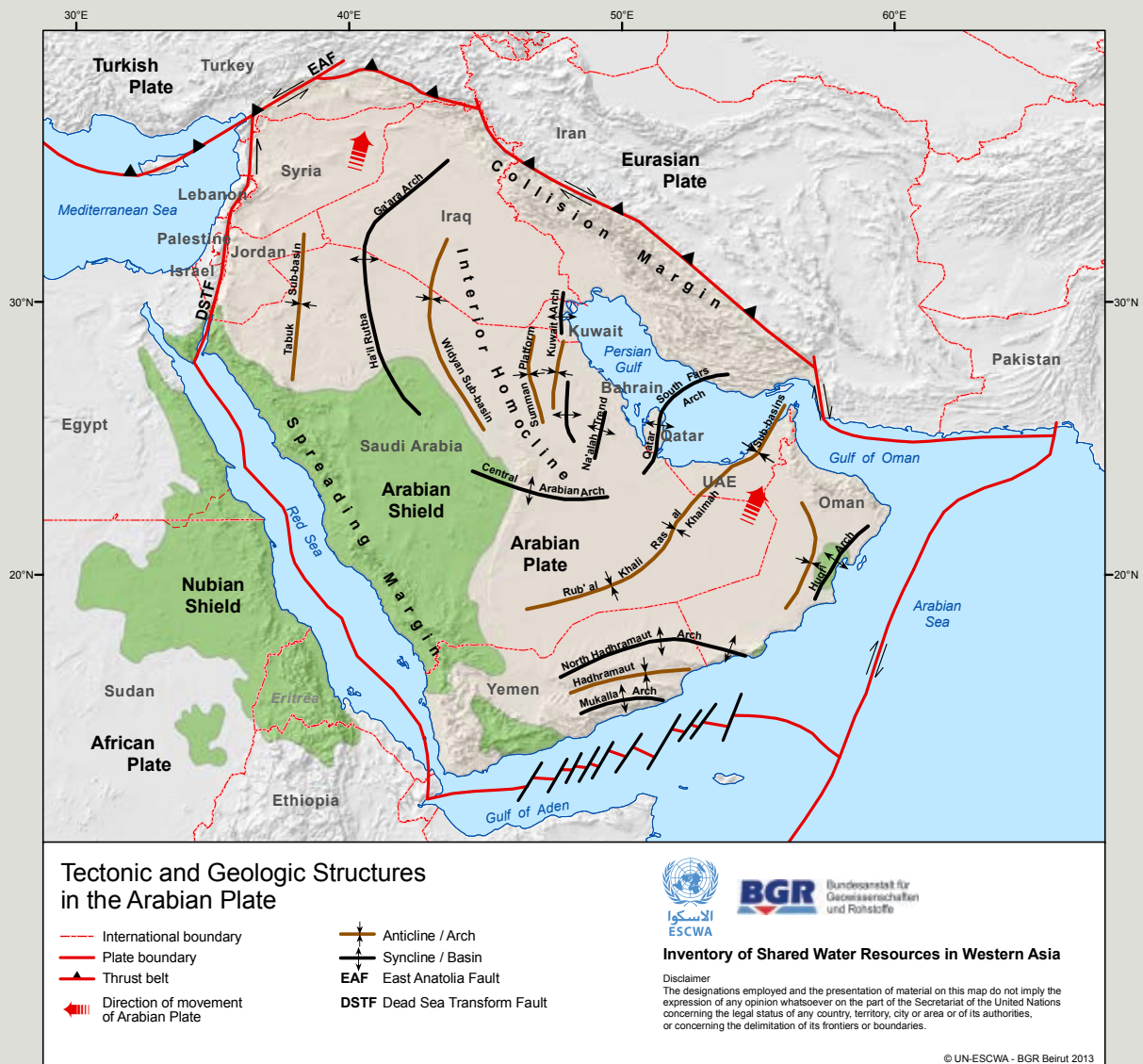
Figure 2. Tectonic and geologic structures in the Arabian Plate
