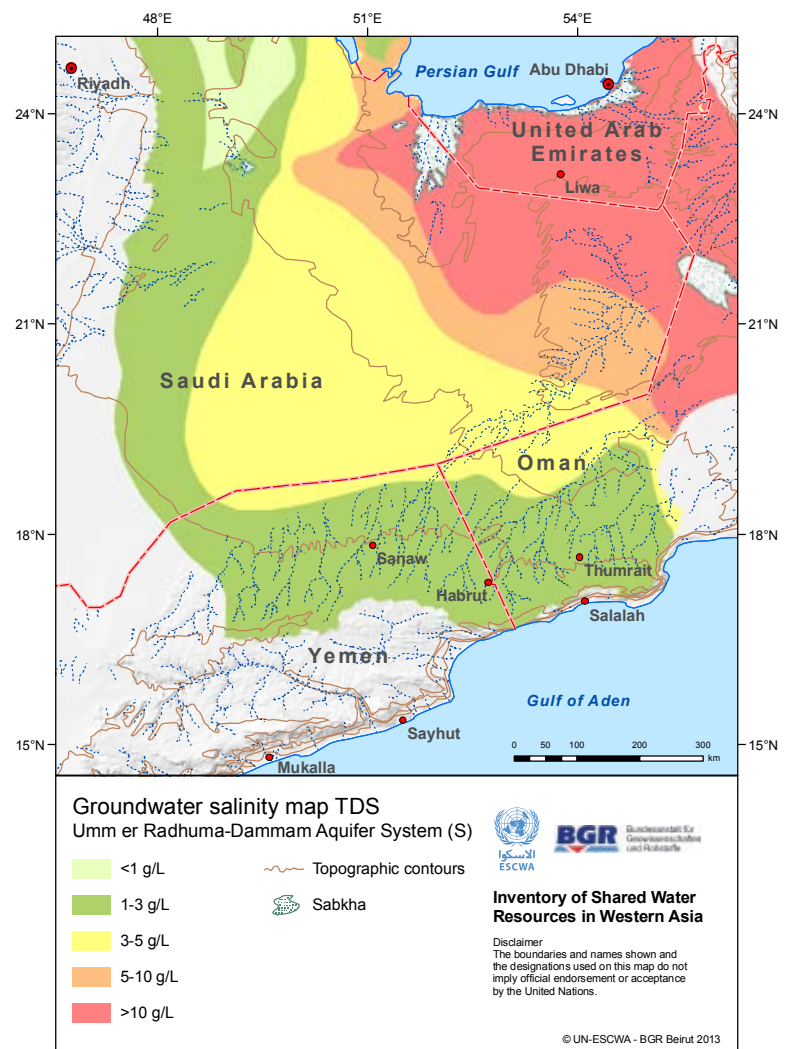
Figure 2. Groundwater salinity map - Umm er Radhuma-Dammam Aquifer System (South)
