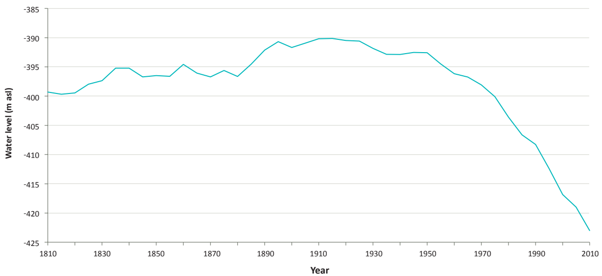
Figure 18. Decline in Dead Sea water levels (1810-2010)
