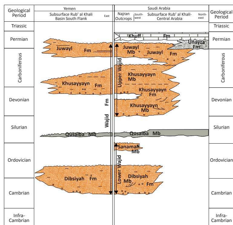
Figure 3. Correlation of the lithostratigraphy of the Wajid Formations in Saudi Arabia and Yemen
