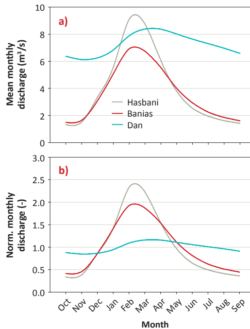
Figure 8. Mean monthly flow regime of the Hasbani, Baniyas and Dan Rivers (1944-2008)
