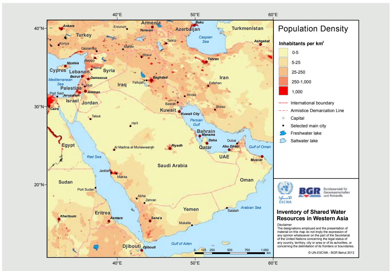
Figure 1. Population density in the Western Asia region
