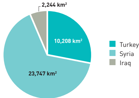
Figure 4. Distribution of the Khabour Basin area
