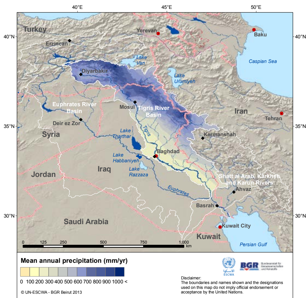
Figure 4. Mean annual precipitation in the Tigris Basin
