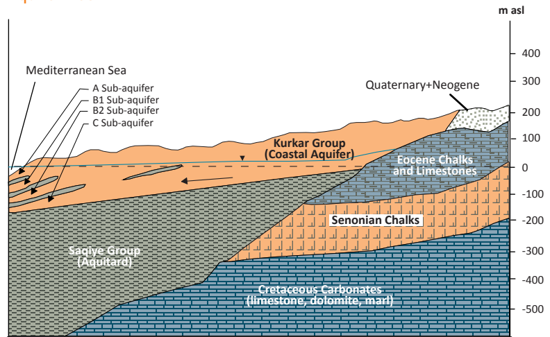
Figure 1. Schematic hydrogeological cross-section of the Coastal Aquifer Basin
