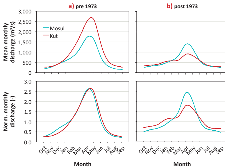
Figure 7. Mean monthly flow regime of the Tigris River at different gauging stations for different time periods (1931-2011)
