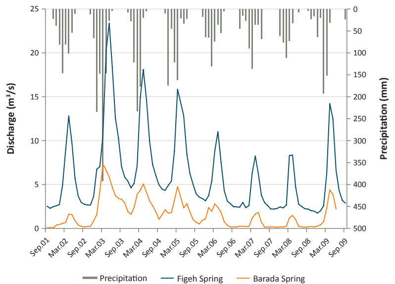
Figure 4. Hydrographs of Figh and Barada Springs and monthly precipitation at Bloudan
