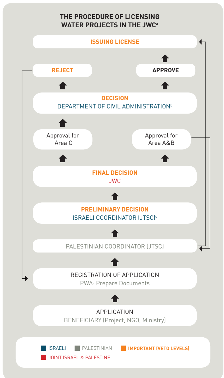
Figure 7. Licensing water projects through the Joint Water Committee
