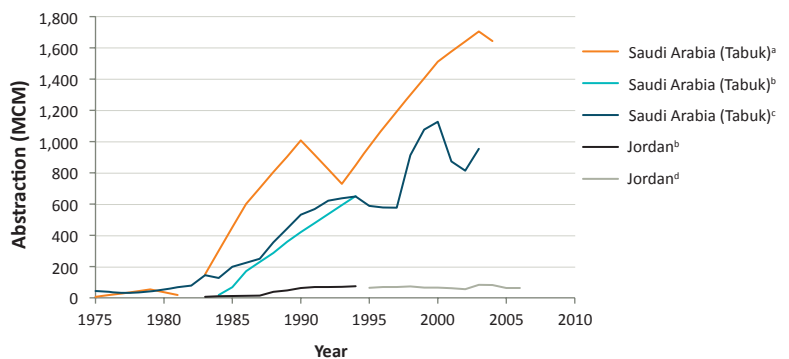
Figure 2. Historical abstraction from the Saq-Ram Aquifer System (West) (1975-2007)
