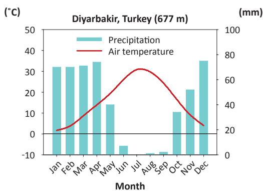
Figure 3. Climate diagrams for Diyarbakir in Turkey, Mosul in Iraq and Baghdad in Iraq
