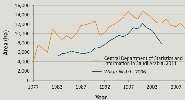
Figure 7. Total cropped area in Najran Province in Saudi Arabia (1977-2009)
