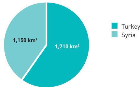
Figure 2. Distribution of the Sajur Basin area
