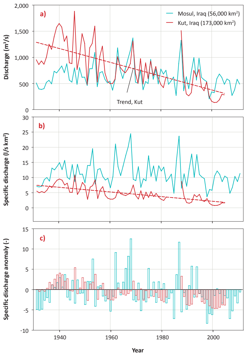
Figure 6. a) Mean annual discharge, b) specific mean annual discharge and c) discharge anomaly time series of the Tigris (1931-2011)
