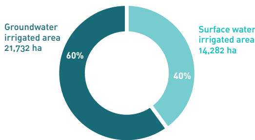
Figure 22. Irrigated area in the Yarmouk Basin in Syria (1999-2009), by source
