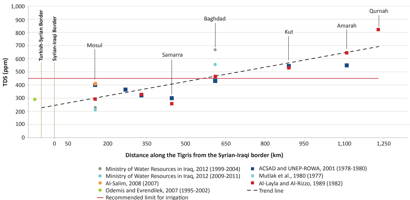
Figure 9. Salinity variations along the Tigris River before 1983 and after 1995
