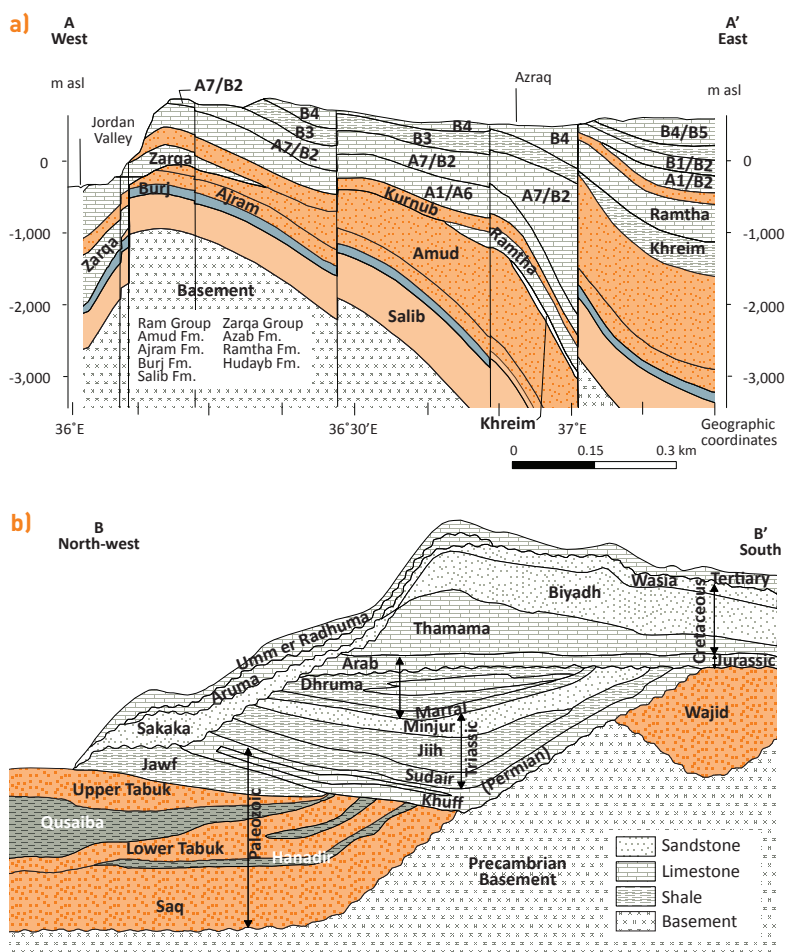
Figure 1. a) Geological cross-section of subsurface stratigraphy of the Ram Aquifer System and overlying formations, b) position of the Saq Aquifer System in relation to major aquifer systems in Saudi Arabia
