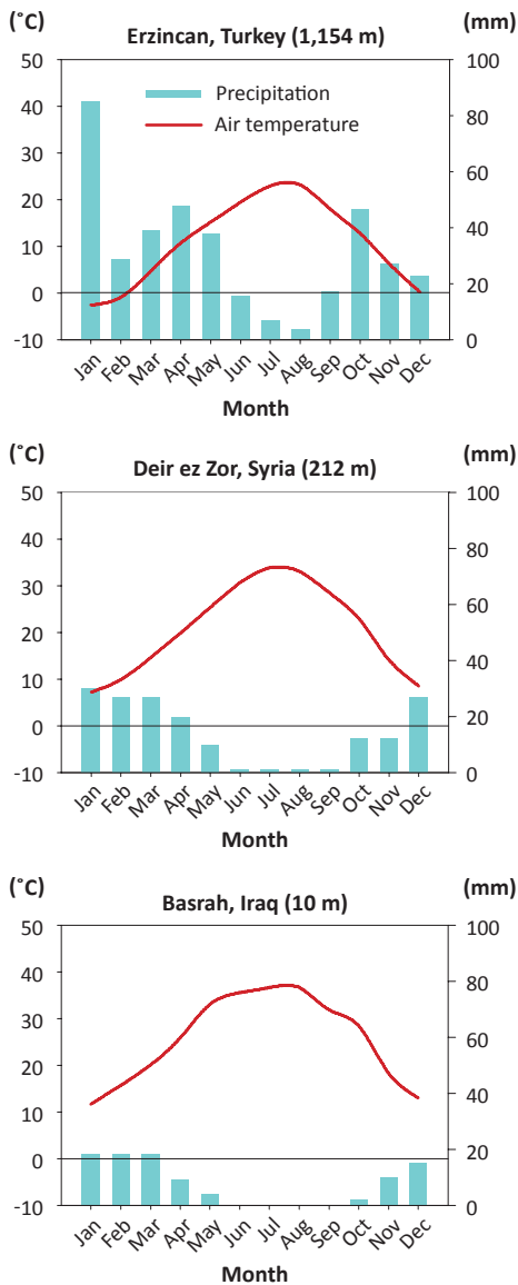
Figure 3. Climate diagrams for Erzinçan in Turkey, Deir ez Zor in Syria, and Basrah in Iraq
