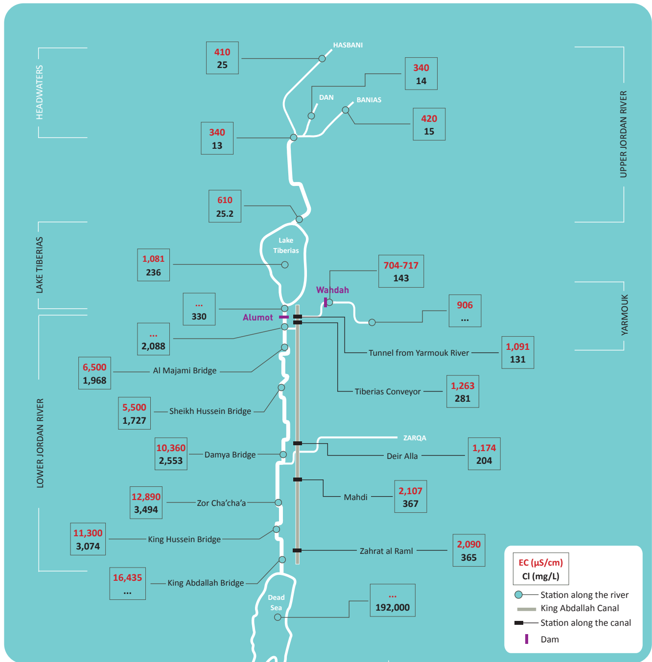
Figure 27. Sketch of salinity levels along the Jordan River and the King Abdullah Canal
