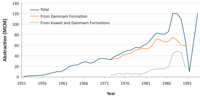
Figure 4. Annual groundwater abstraction from well fields in Kuwait
