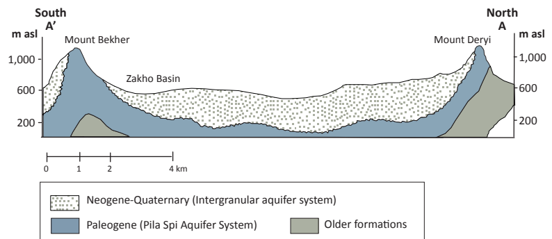
Figure 5. Hydrogeological cross-section of the Zakho Basin
