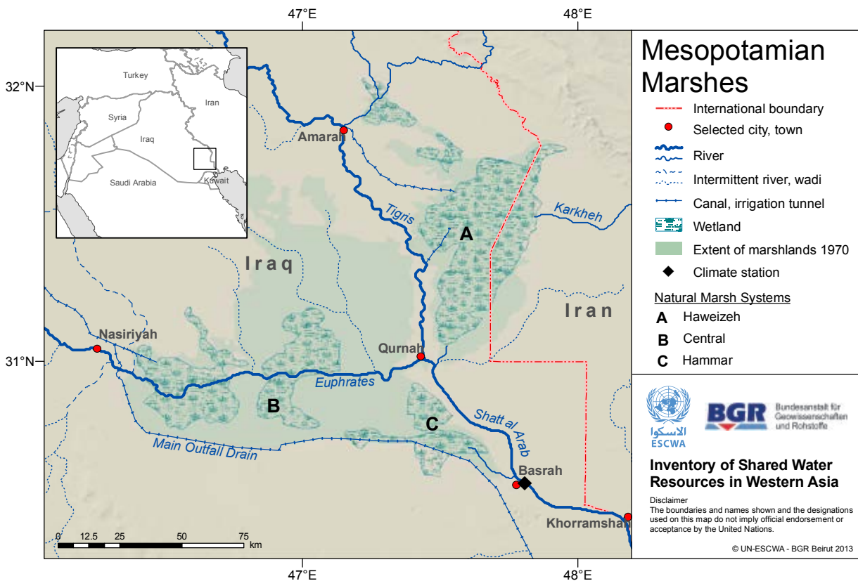
Figure 10. The Mesopotamian Marshes in 2012
