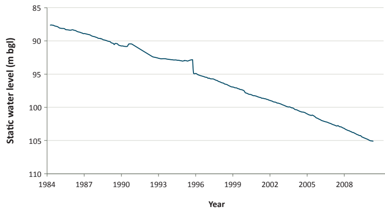
Figure 5. Groundwater decline in the Ram Aquifer in the South Wadi Araba Basin in Jordan (1984-2010)
