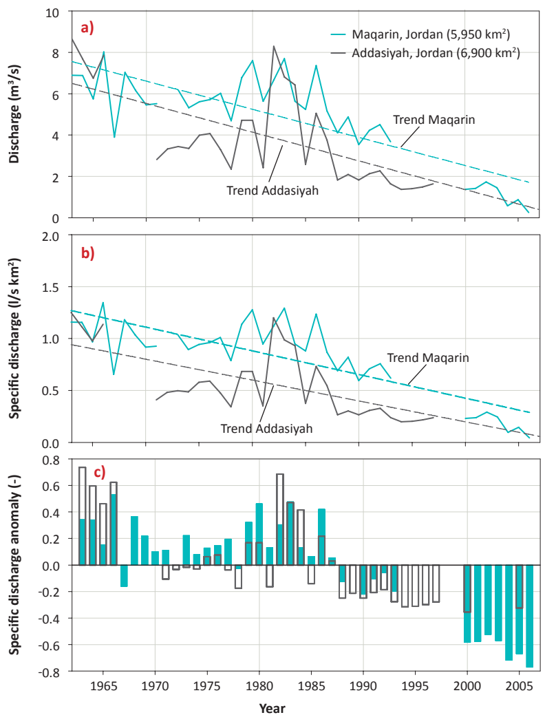
Figure 14. a) Mean annual discharge, b) specific mean annual discharge and c) discharge anomaly time series of the Yarmouk River (1963-2006)
