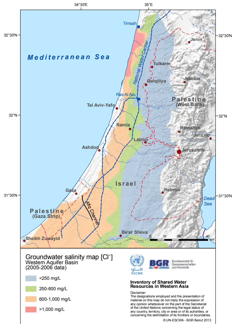
Figure 4. Groundwater salinity map - Western Aquifer Basin
