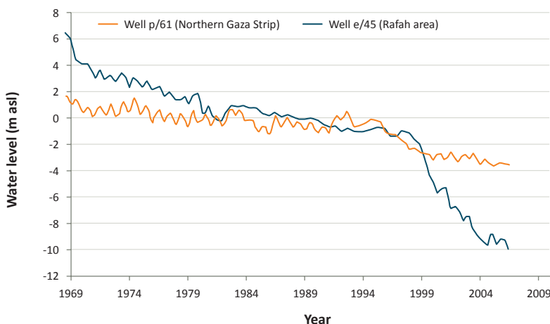
Figure 5. Groundwater levels in two wells in the Gaza Strip
