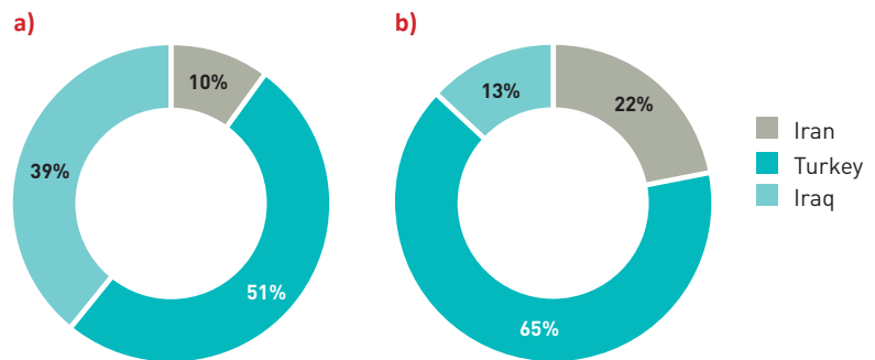
Figure 5. Riparian contribution to annual discharge of the Tigris based on published data
