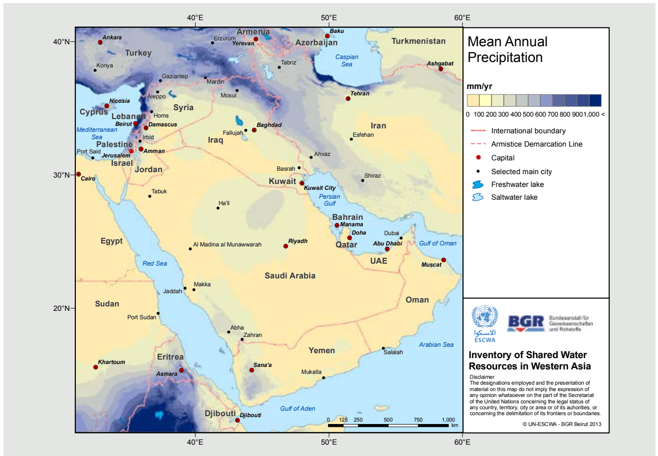
Figure 3. Mean annual precipitation distribution across the Western Asia region
