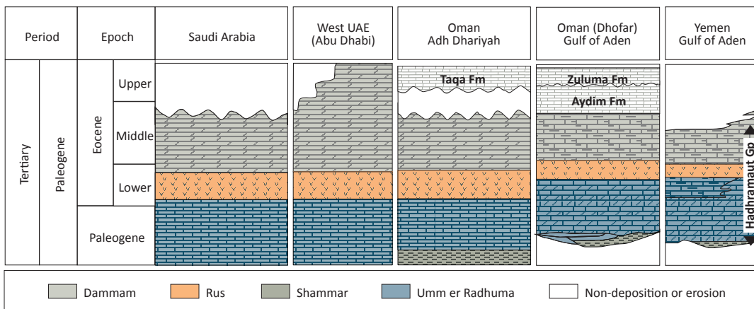
Figure 1. Lithostratigraphy of the Umm er Radhuma-Dammam Aquifer System (South)
