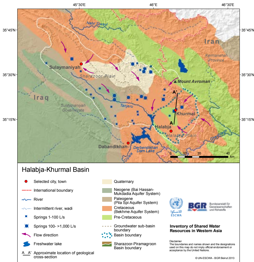
Figure 1. Overview Map of the Halabja-Khurmāl Basin
